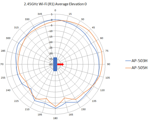
2.45 GHz Wi-Fi (antennas 0, 1)
