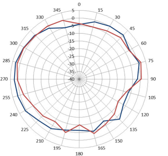
Elevation plane (front view) 5.500 GHz
