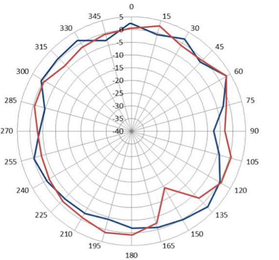
Horizontal or azimuth plane (top view) 5.500 GHz
