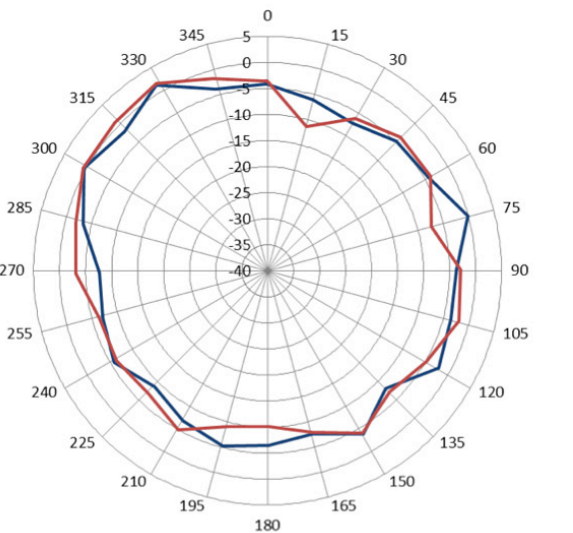
Elevation plane (side view) 5.500 GHz
